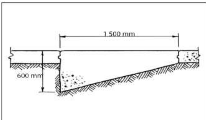
Figure 5: Anchor block
