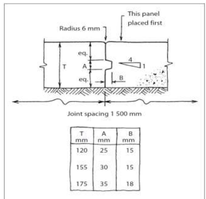
Figure 3: Longitudinal section through road showing keyed joint
