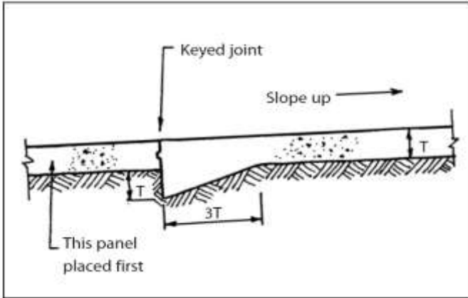
Figure 4: Panel anchor
